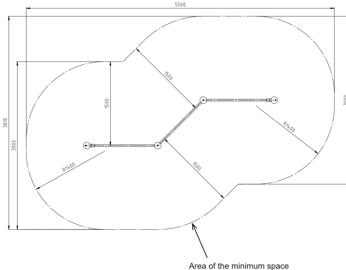
Diagram 3: Top view
